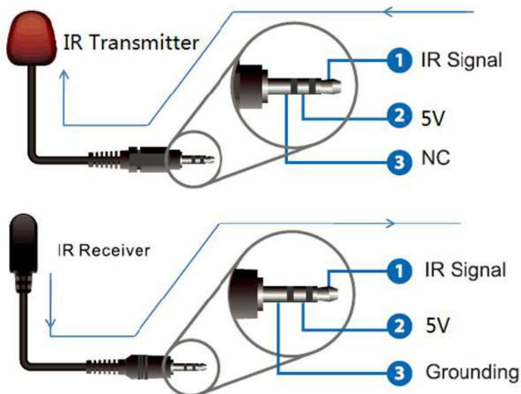
IR extender connectors (not as accessories)
