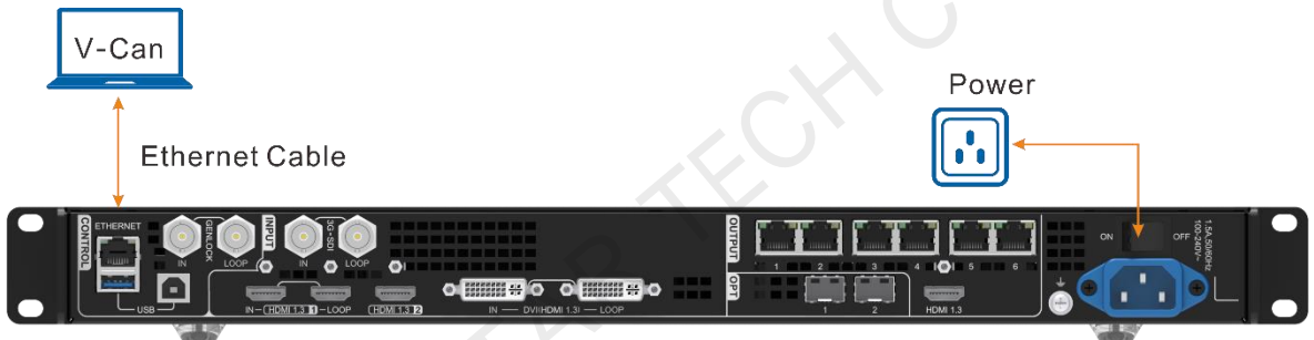
Figure 6-1 Hardware connection
